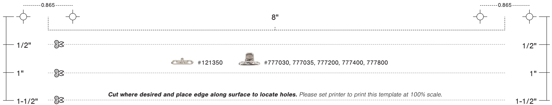
Studs With Holes 0.865" Apart Pattern Template
